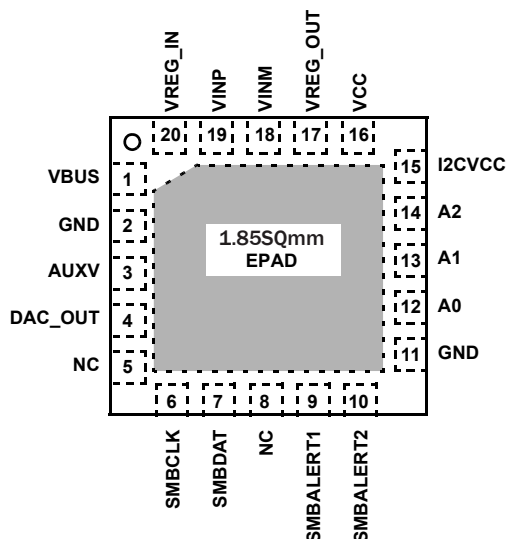
ISL28025FR – 20 lead QFN 4x4 (1.85SQmm EPAD)
