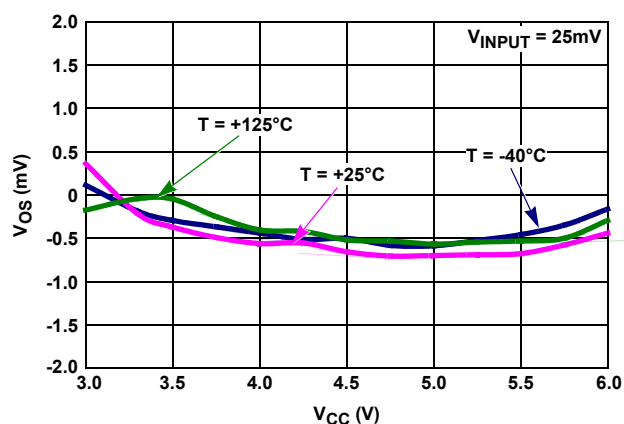
FIGURE 30. AUXILIARY V_{BUS} V_{OS} vs V_{CC}
