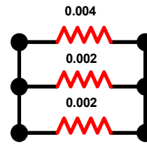
FIGURE 84. INCREASING THE NUMBER OF SHUNT RESISTORS IN PARALLEL TO CREATE A SHUNT RESISTOR VALUE REDUCES THE POWER DISSIPATED BY EACH SHUNT RESISTOR
