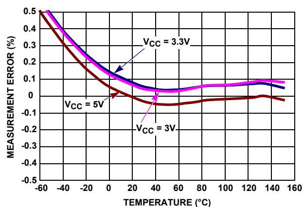
FIGURE 36. AUXILIARY V_{BUS} MEASUREMENT ERROR vs TEMPERATURE
