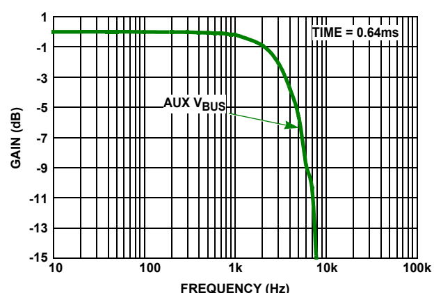
FIGURE 28. AUXILIARY V_{SHUNT} AND V_{BUS} vs FREQUENCY
