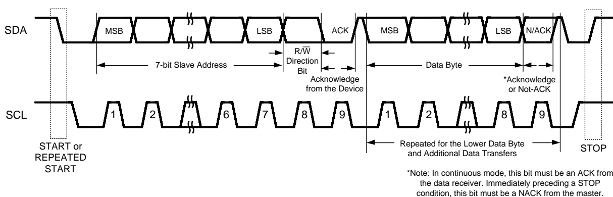
Figure 21. Basic Operation.
