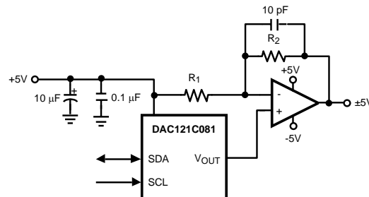
Figure 31. Bipolar Operation
