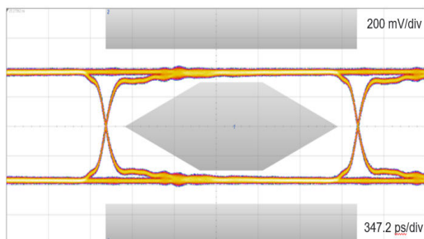
Figure 9. USB2.0 480 Mbps eye diagram with device
