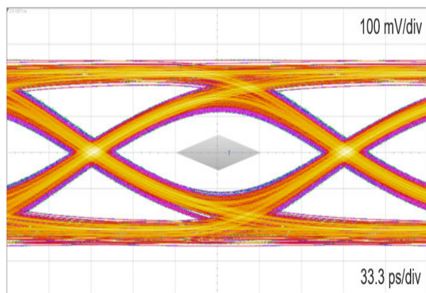
Figure 11. USB3.2 Gen 1 5.0 Gbps eye diagram with ECMF04-4HSM10 (with worst cable and equalizer)
