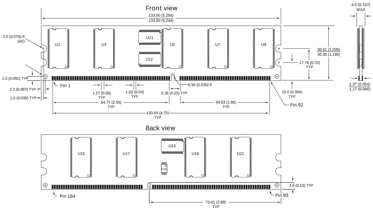
Figure 5: 184-Pin DDR RDIMM – Standard-Height Layout
