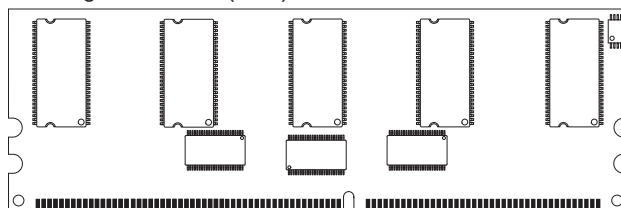
Figure 2: Standard-Height Layout (MO-206-CA R/C L)
