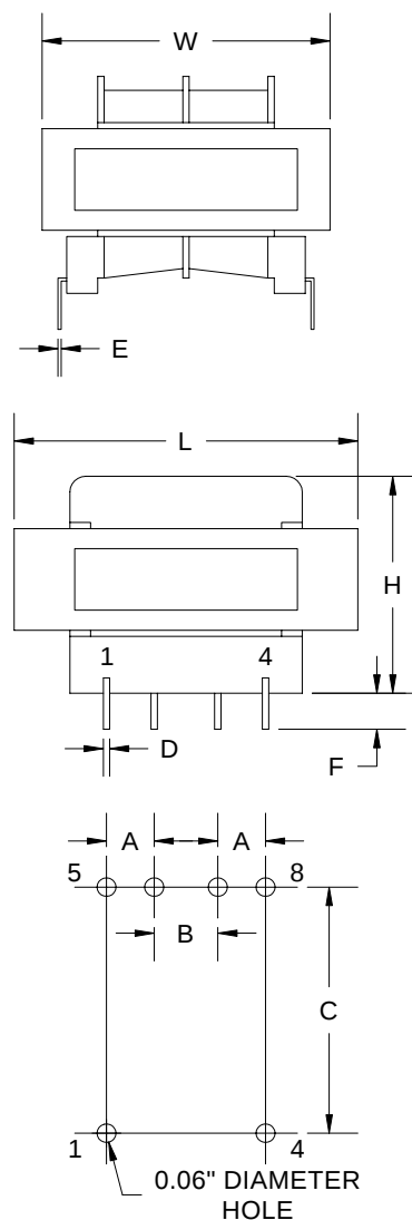
Board Layout
