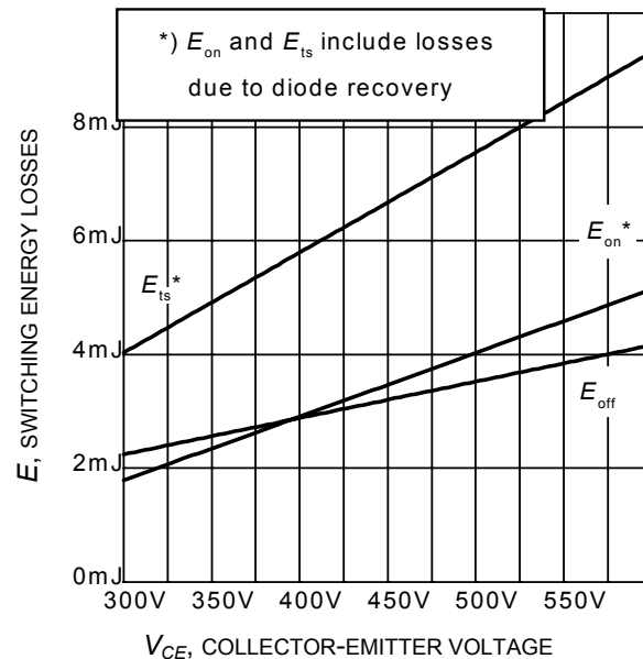
Figure 16. Typical switching energy losses as a function of collector emitter voltage (inductive load, T_J = 175^\circ\text{C} , V_{GE} = 0/15\text{V} , I_C = 75\text{A} , R_G = 5\Omega , Dynamic test circuit in Figure E)
