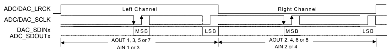
Figure 16. Right-Justified Format
