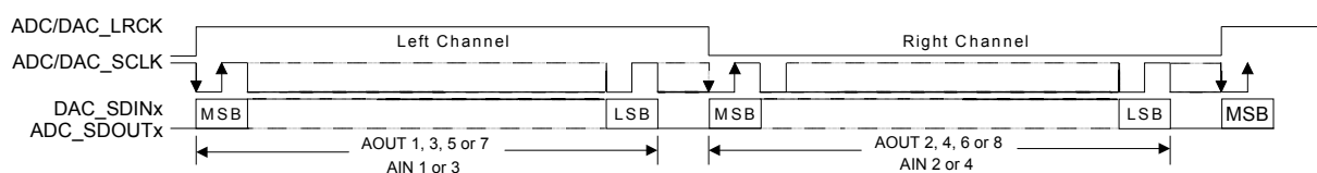
Figure 15. Left-Justified Format
