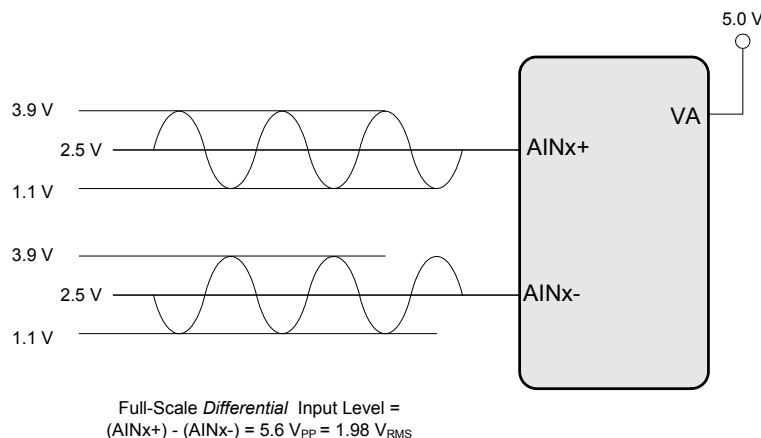
Figure 10. Full-Scale Input
