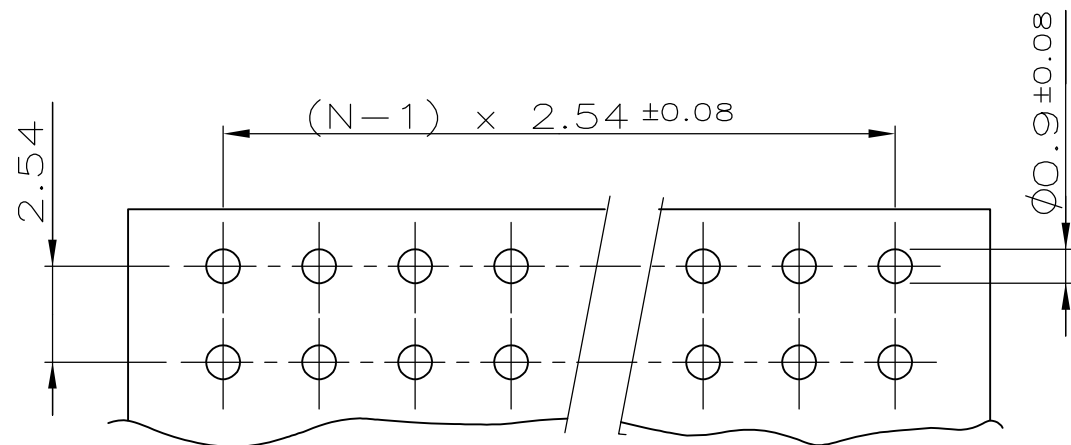
P.C.-BOARD HOLE-PATTERN
