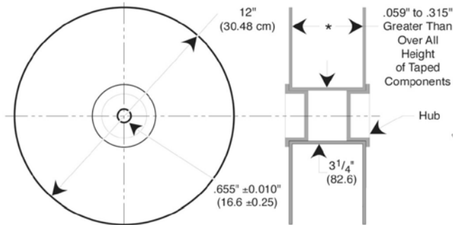
Figure 3: Standard Reel
