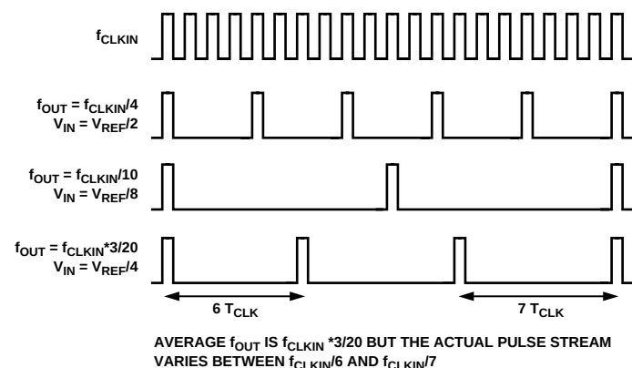
Figure 7. AD7741/AD7742 Frequency Output Waveforms
