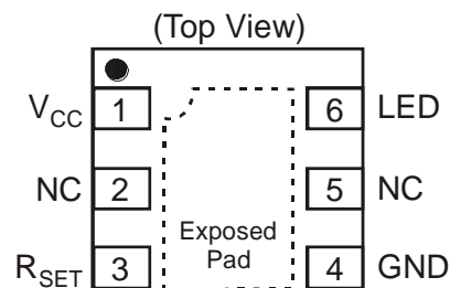
U-DFN3030-6
