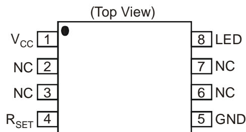
MSOP-8EP
