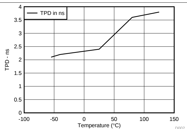
Figure 2. TPD Across Temperature at 3.3 V
