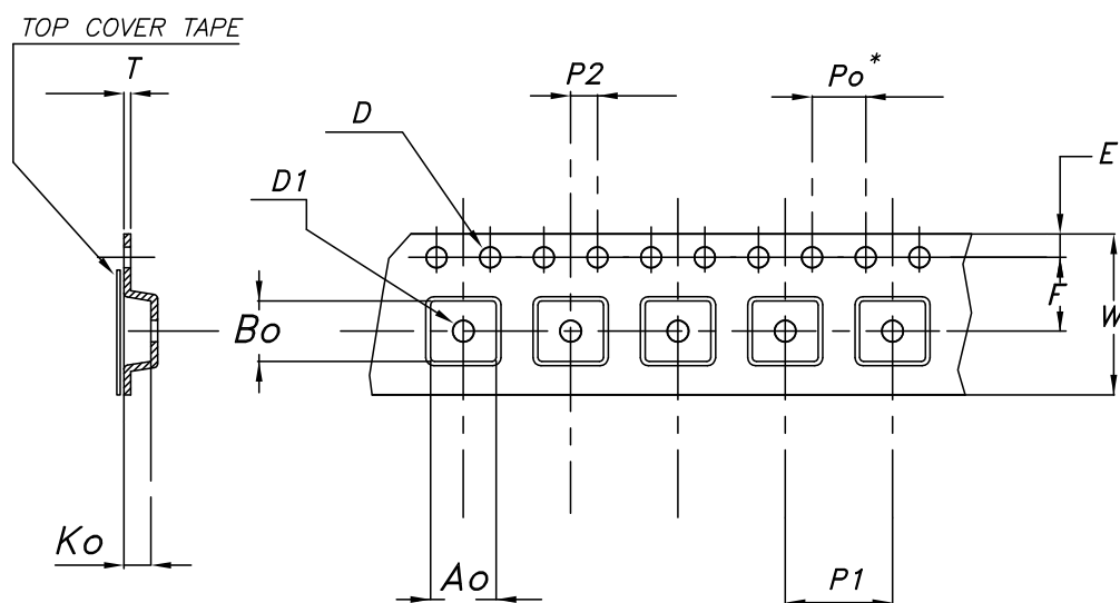
Figure 42. SOT-89 device orientation
