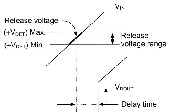
Figure 30 Release Voltage
