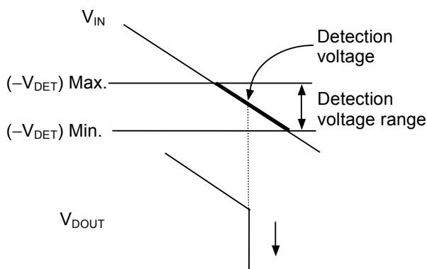
Figure 29 Detection Voltage
