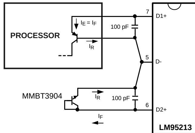
Figure 16. Thermal Diode Current Paths
