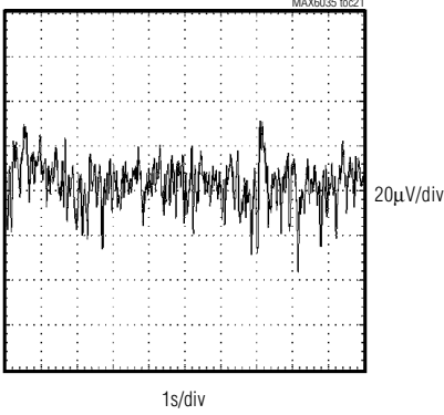
MAX6035 0.1Hz to 10Hz OUTPUT NOISE ( V_{OUT} = 5V )
