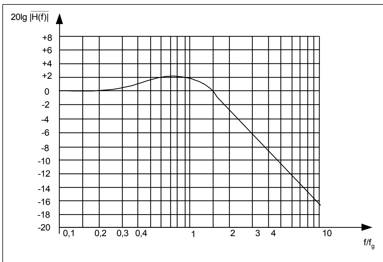
Figure 8 APLL - Jitter Transfer Function
