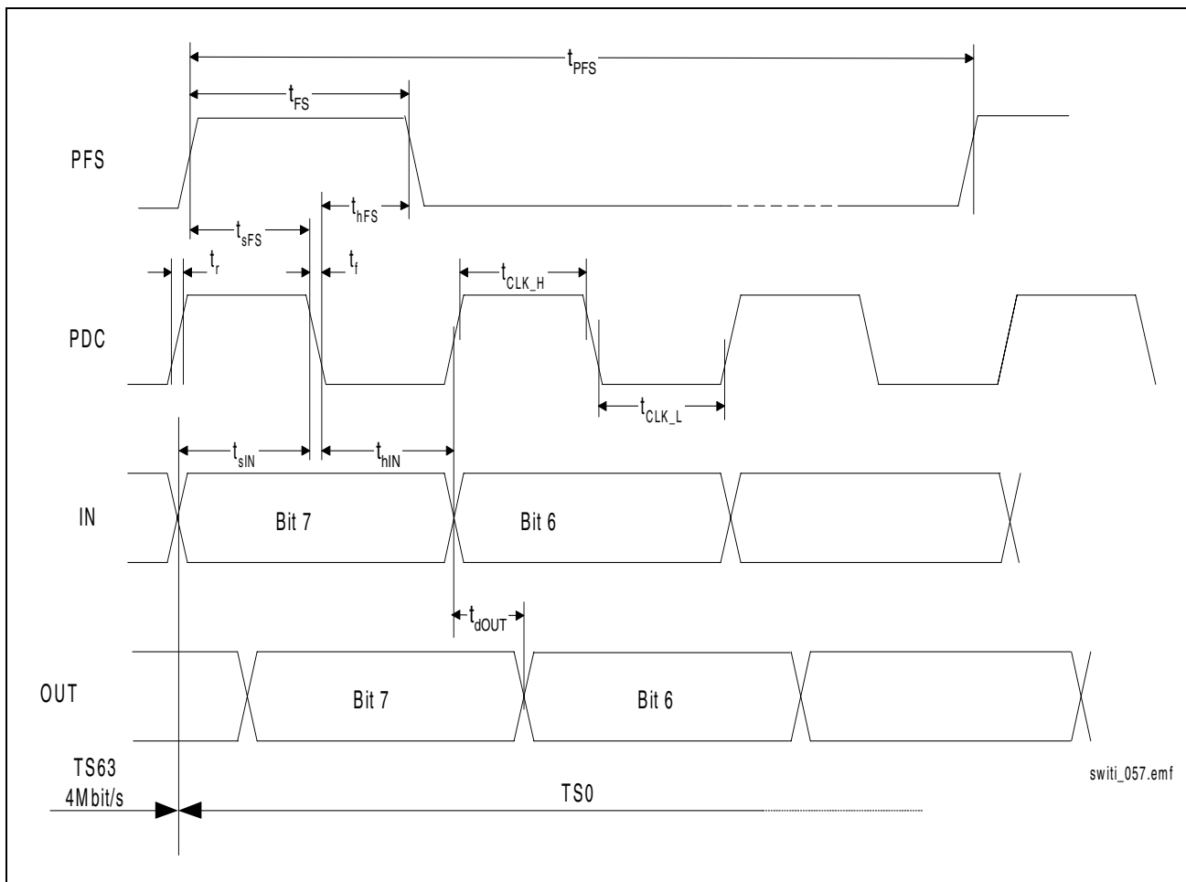
Figure 31 PCM Timing
