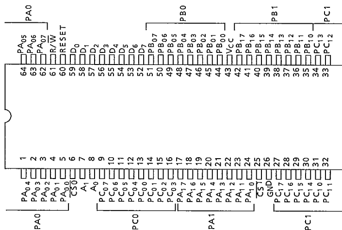
TMP82C265BF-2/TMP82C265BF-10
