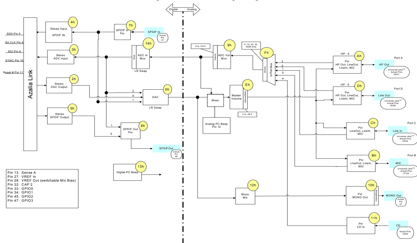
Figure 3. STAC9250 Widget Diagram
