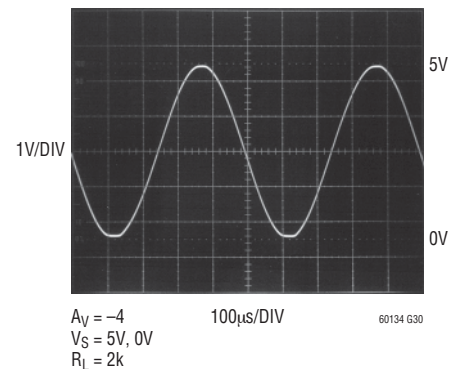
Rail-to-Rail Output Swing
