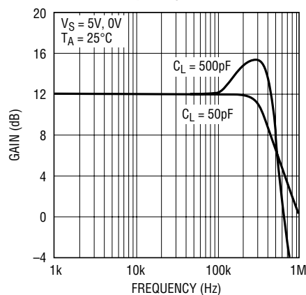
Gain vs Frequency, A_V = -4
