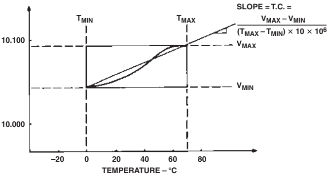
Figure 9. Typical AD587L Temperature Drift
