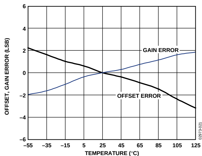
Figure 22. Offset and Gain Error vs. Temperature
