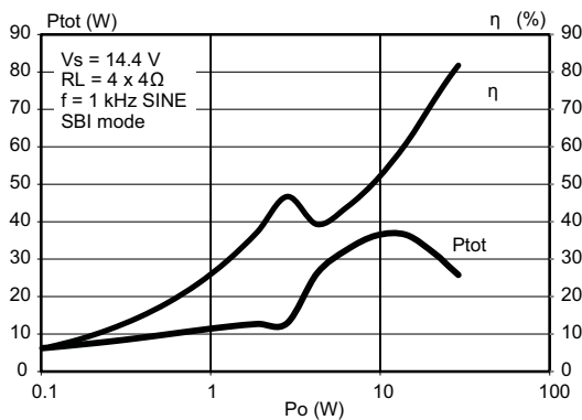
Figure 21. Total power dissipation & efficiency vs. Po (4 \Omega , SBI, Sine)
