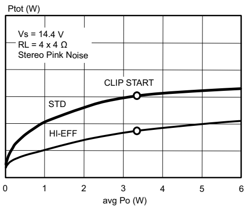
Figure 22. Power dissipation vs. average Po (audio program simulation, 4 \Omega )
