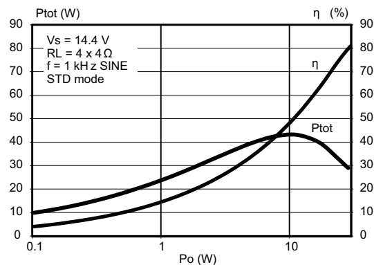
Figure 20. Total power dissipation & efficiency vs. Po (4 \Omega , STD, Sine)
