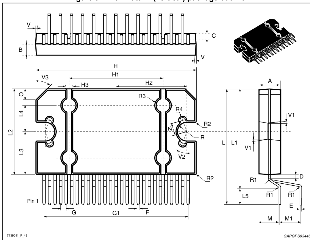
Figure 34. Flexiwatt 27 (vertical) package outline
