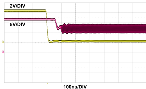
FIGURE 39. POWER-UP TIME
