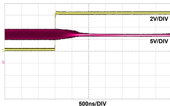
FIGURE 40. POWER-DOWN TIME
