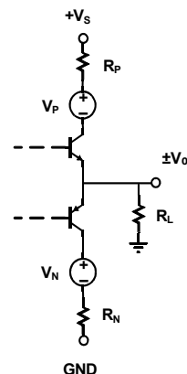
FIGURE 51. HEADROOM MODEL
