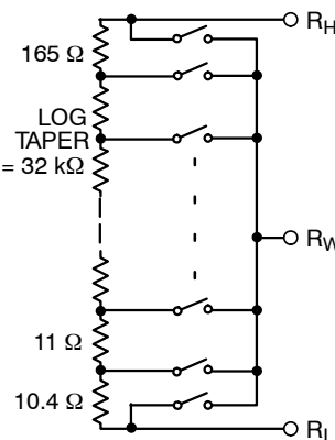
Figure 3. Potentiometer Schematic
