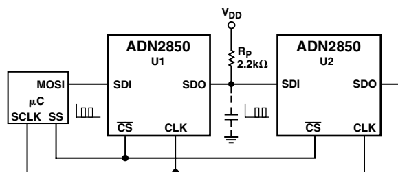
Figure 4. Daisy-Chain Configuration
