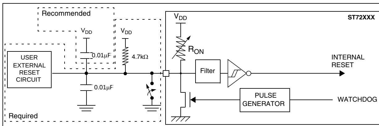
Figure 90. RESET pin protection when LVD is disabled. 1)2)3)
