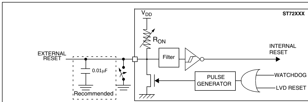
Figure 90. RESET pin protection when LVD is disabled. 1)2)3)
