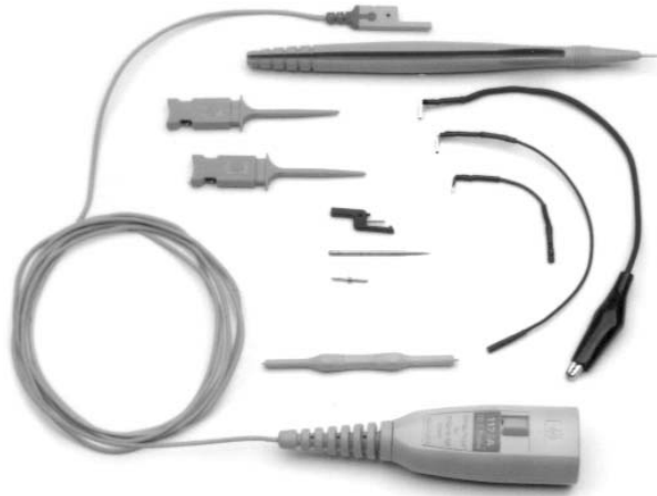
Figure 2.7. Agilent 117XA family probes for fine-pitch ICs, surface mount devices, and dense circuit boards.
