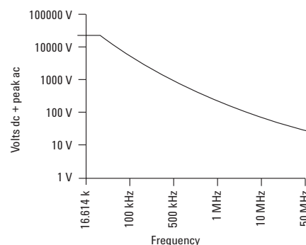
Figure 6.6. Derating curve showing bandwidth characteristics of the N2771A probe.
