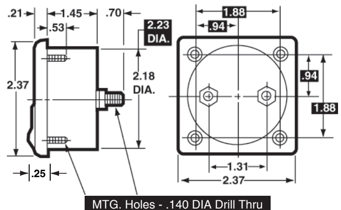
2-1/2"-Model 127 & 127T, 147, 157, & 187
