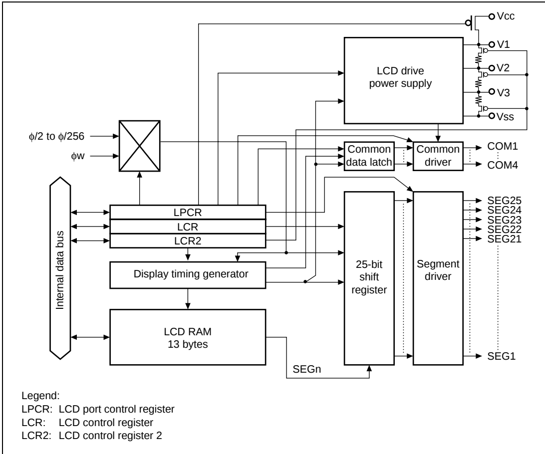
Figure 13.1(2) Block Diagram of LCD Controller/Driver (H8/38104 Group)
