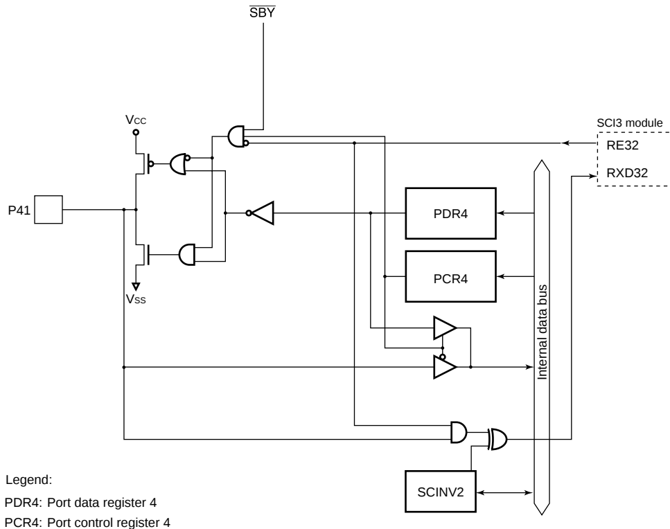
Figure B.2(c) Port 4 Block Diagram (Pin P41)
