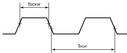
Figure 17.4 SCK3 Input Clock Timing
