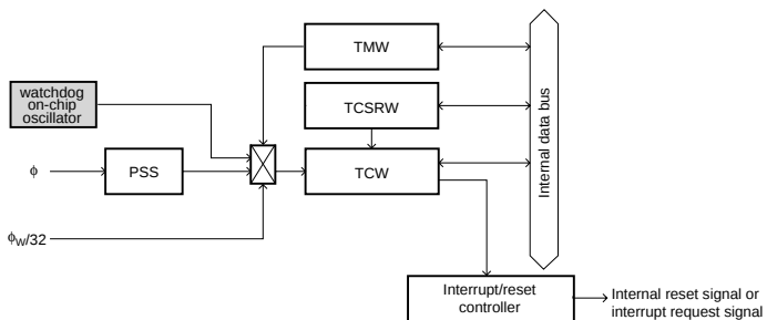
Figure 9.12(2) Block Diagram of Watchdog Timer (H8/38104 Group)
