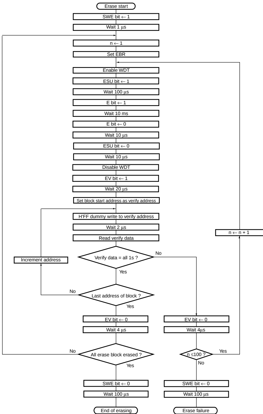
Figure 6.11 Erase/Eraser-Verify Flowchart
