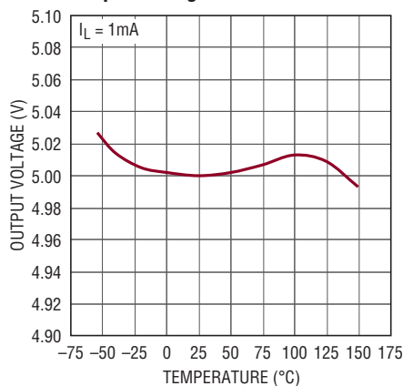
Output Voltage-LT3055-5
