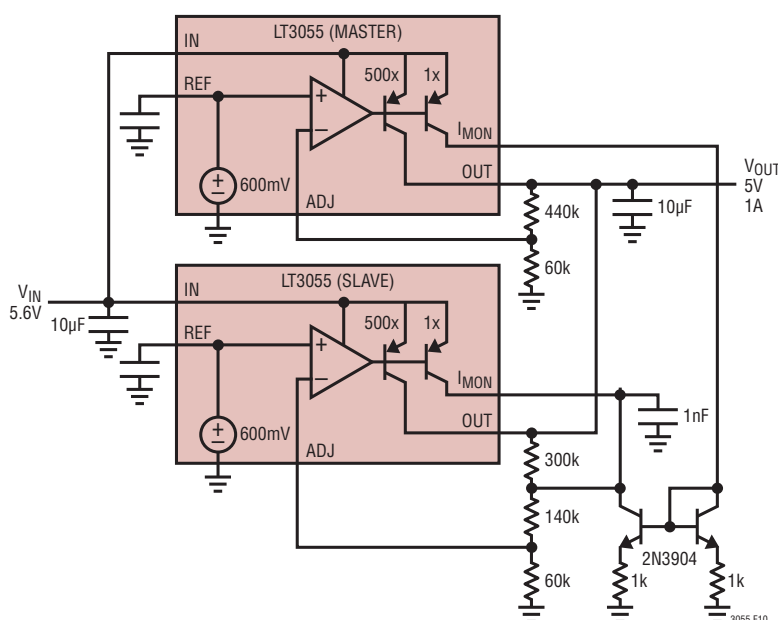
Figure 10. Paralleling Devices
