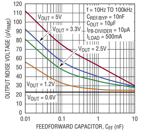
RMS Output Noise vs Feedforward Capacitor ( C_{\text{FF}} )
