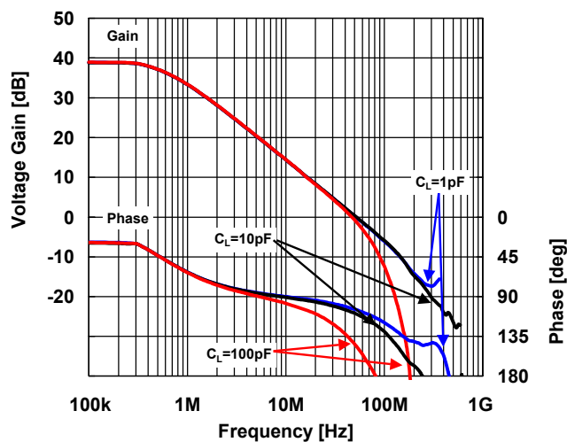
Gain/Phase vs. Frequency (Load Capacitance) V^+/V^-=\pm 15\text{V} , V_{IN}=0.02\text{V}_{pp} , G_v=40\text{dB} , R_I=50\Omega , R_F=1.98\text{k}\Omega , R_G=20\Omega , C_F=0\text{F} , R_L=500\Omega , T_a=+25^\circ\text{C}
