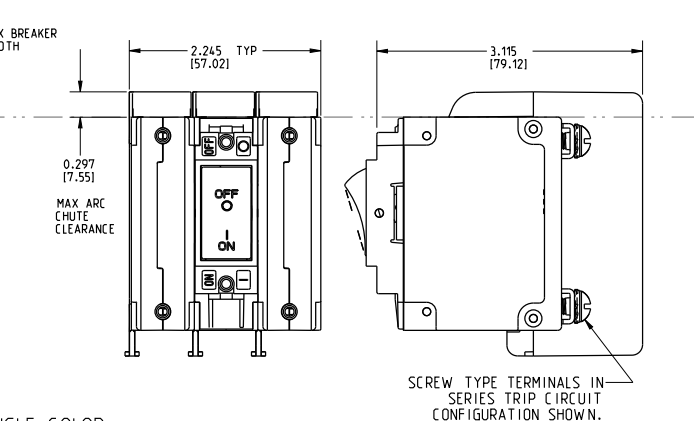
3-POLE (CF3,CG3,C13,C23) w/ ARC CHUTE BARRIER
