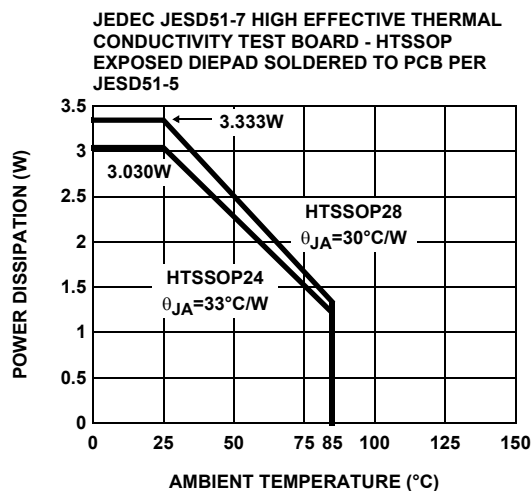
FIGURE 29. PACKAGE POWER DISSIPATION vs AMBIENT TEMPERATURE
