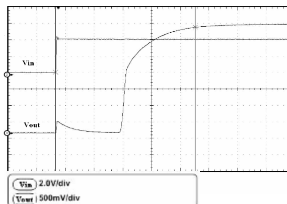
Figure 13. Enable transient
