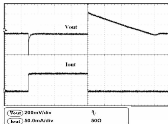
Figure 11. Load transient
