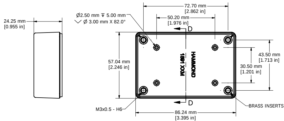
SIDE VIEW OF BOX
