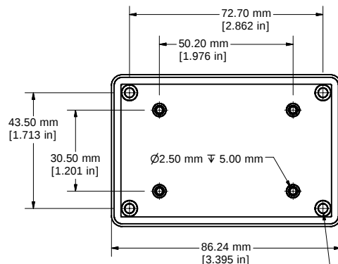
BOTTOM VIEW OF LID
