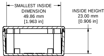
SECTION E-E
