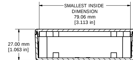
SECTION F-F
