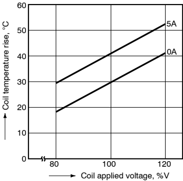
3.-(3) Coil temperature rise (2a type)
