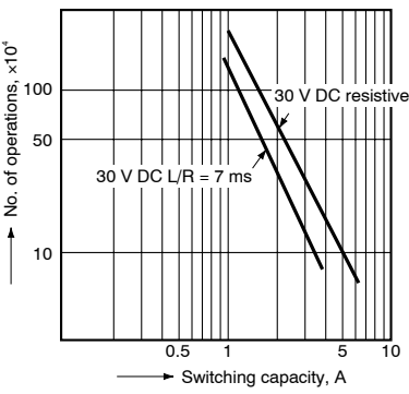
2.-(2) Life curve (1a1b type)
