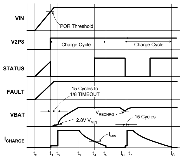
FIGURE 20. TYPICAL OPERATING WAVEFORMS
