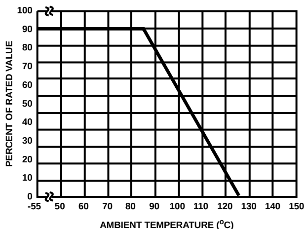
FIGURE 1. CURRENT, ENERGY AND POWER DERATING CURVE
