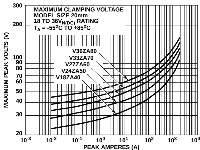
FIGURE 12. CLAMPING VOLTAGE FOR V18ZA40 - V36ZA80
