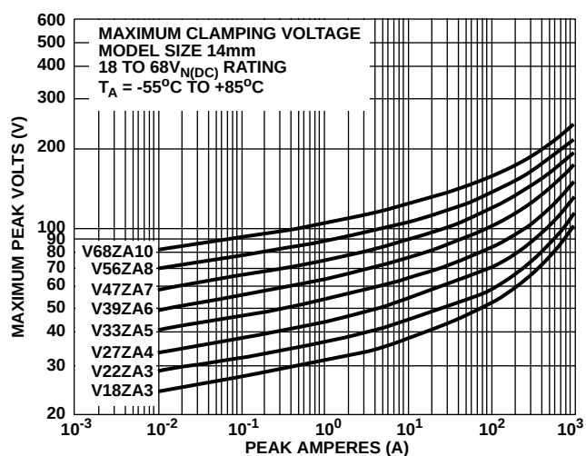
FIGURE 10. CLAMPING VOLTAGE FOR V18ZA3 - V68ZA10
