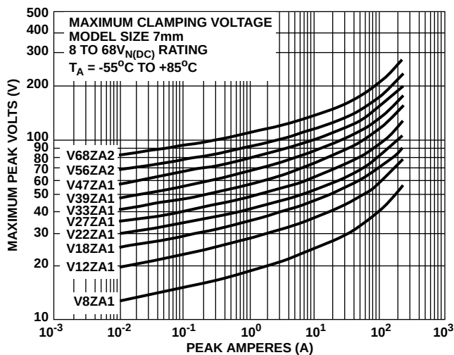
FIGURE 6. CLAMPING VOLTAGE FOR V8ZA1 - V68ZA2
