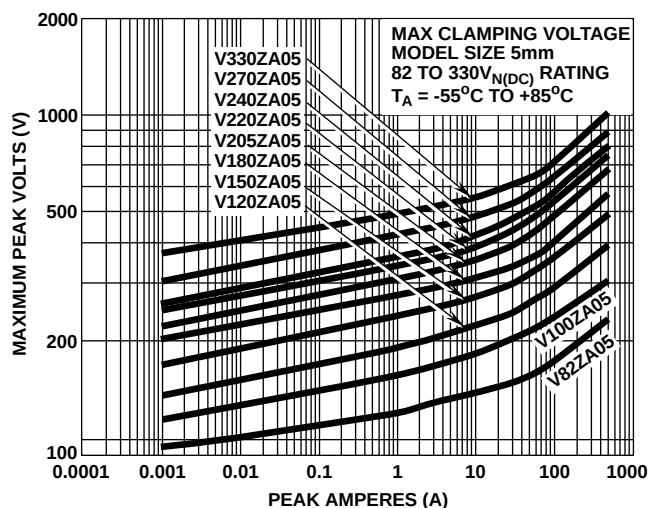
FIGURE 4. CLAMPING VOLTAGE FOR V82ZA05 - V330ZA05
