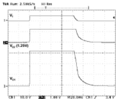
Figure 33: Start-Up Transient
