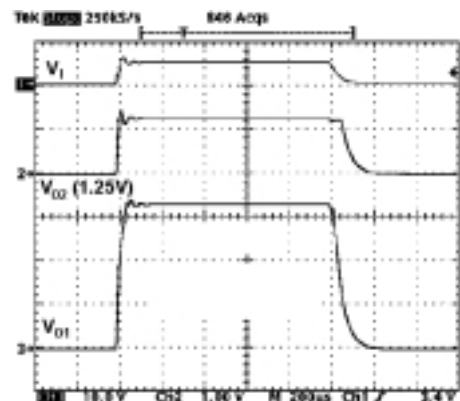
Figure 34: Start-Up Transient
