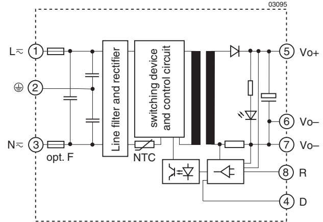
Fig. 2 Block diagram LOK4140, LOK4240 and LOK4740 (battery charger versions) and LOK4001- 2RLD.
