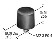
B AT413 .315" (8.0mm) Diameter Screw-on Cap
