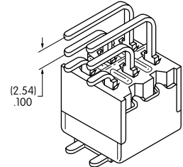
45 .100" (2.54mm) Vertical PC
