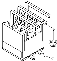
30 Right Angle PC with .646" (16.4mm) Support to Terminal
