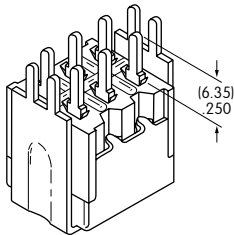
13 .250" (6.35mm) Straight PC with Bracket
