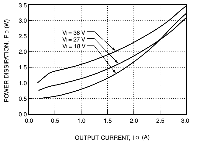
Figure 51. LC010F Typical Power Dissipation vs. Output Current at T_c = 25^\circ\text{C}
