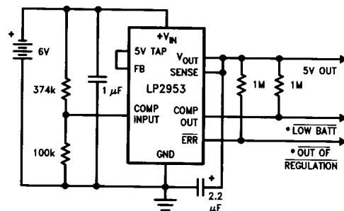
5V Regulator with Error Flags for LOW BATTERY and OUT OF REGULATION
