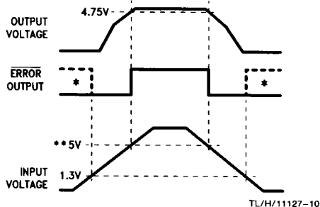
FIGURE 4. ERROR Output Timing
