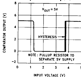
Comparator Outputs
