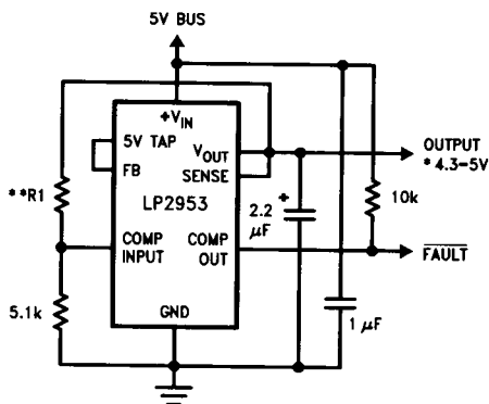
5V Current Limiter with Load Fault Indicator
