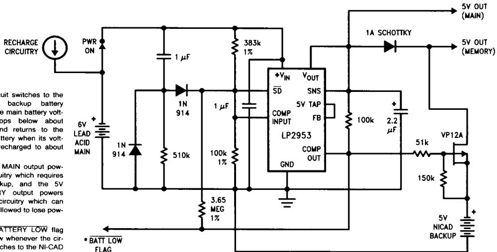
5V Battery Powered Supply with Backup and Low Battery Flag
