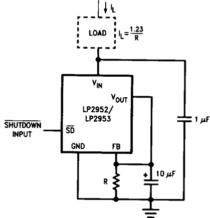
Low T.C. Current Sink
