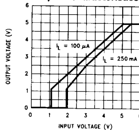
Dropout Characteristics
