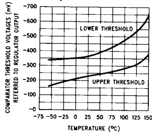
Dropout Detection Comparator Threshold Voltages
