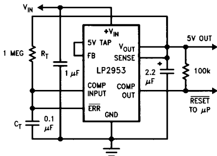
5V Regulator with Timed Power-On Reset
