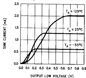
Comparator Sink Current
