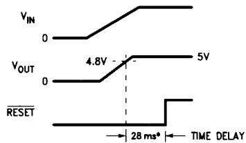
Timing Diagram for Timed Power-On Reset
