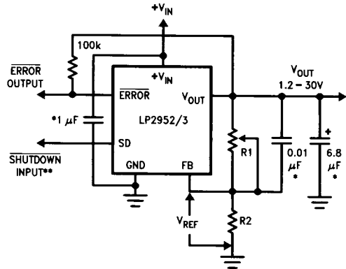
FIGURE 3. Adjustable Regulator
