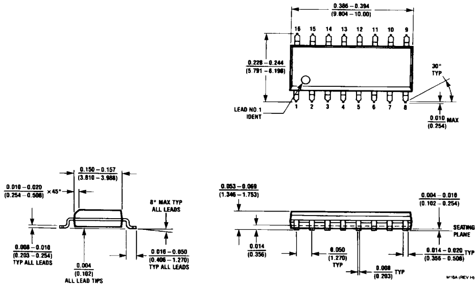
16-Pin Surface Mount Order Number LP2952IM, LP2952AIM, LP2953IM or LP2953AIM NS Package Number M16A
