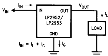
FIGURE 1. Current/Voltage Diagram
