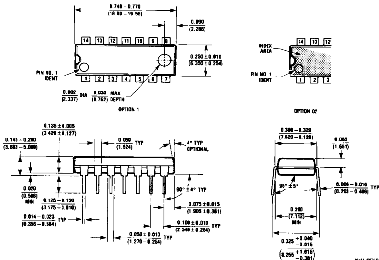
14-Pin Molded DIP Order Number LP2952IN or LP2952AIN NS Package Number N14A
