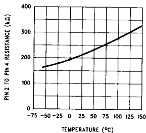
Divider Resistance
