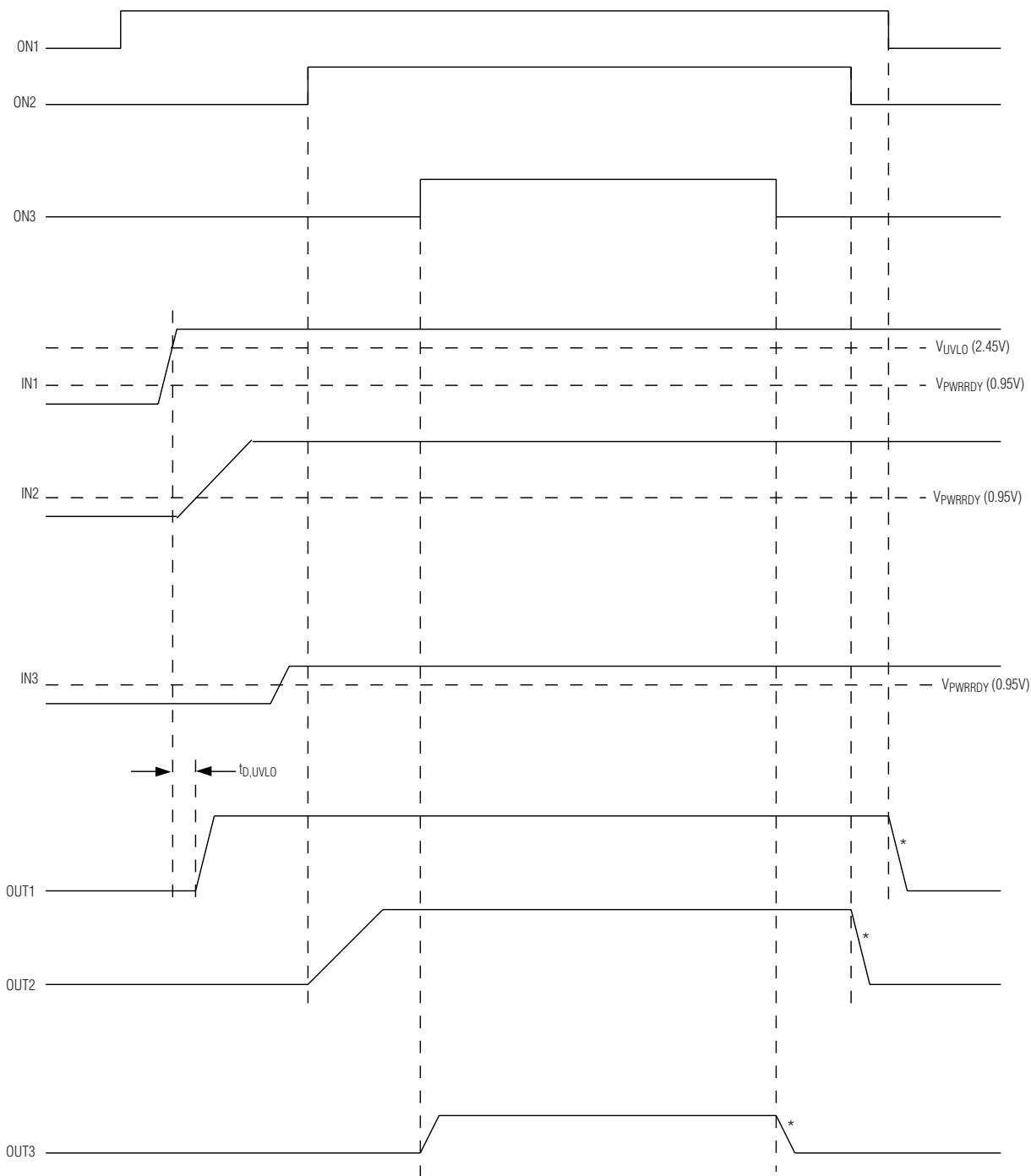
Figure 5. Independent-Mode Timing Diagram
