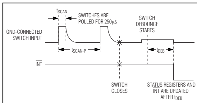
Figure 6. Switch Sampling in Scan Mode
