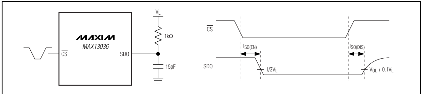
Figure 2. SDO Enable/Disable Test Circuit and Timing Diagram
