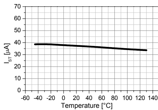
Figure 7. Start-up Supply Current vs. Temp.
