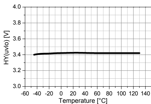
Figure 6. UVLO Hysteresis vs. Temp.
