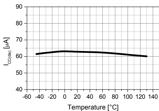
Figure 10. I_{CCDIS} at Disable vs. Temp.
