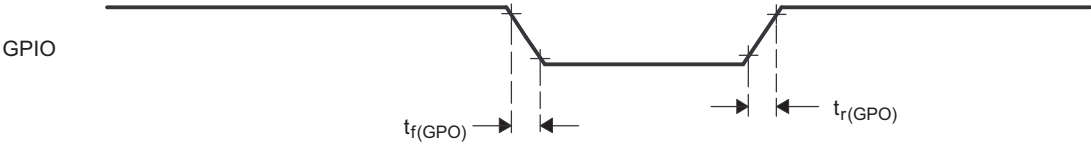
Figure 6-41. General-Purpose Output Timing
