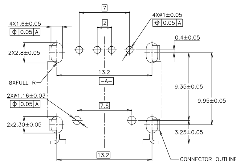
REFERENCE PCB LAYOUT (MOUNTING SIDE)
