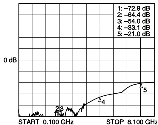
S 12 -FREQUENCY
