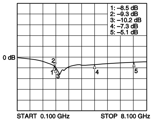
S 11 -FREQUENCY
